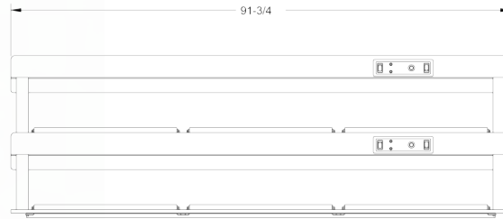
Model HF91-2
