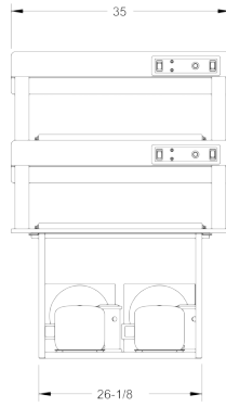
Model HF35-2
