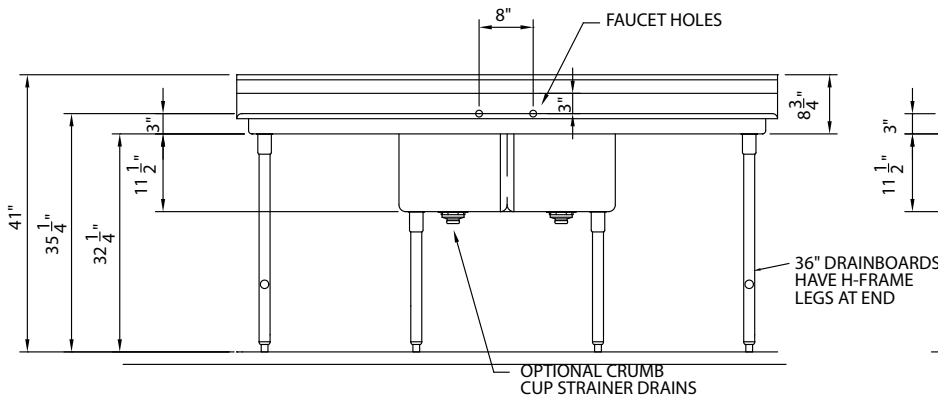
FRONT VIEW
