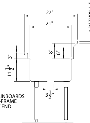
SECTION VIEW
