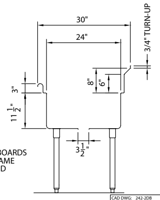
SECTION VIEW
