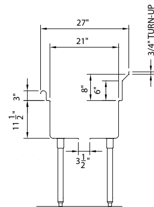
SECTION VIEW
