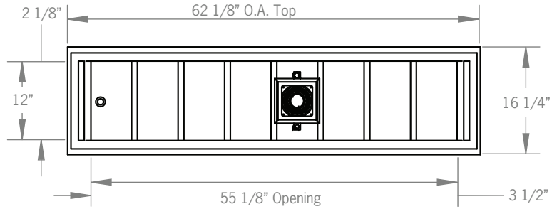
KRD-62S Plan View
