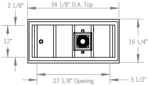
KRD-34S Plan View
