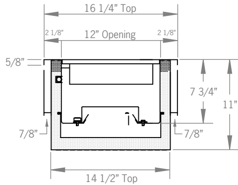
Flat Rail Section View
