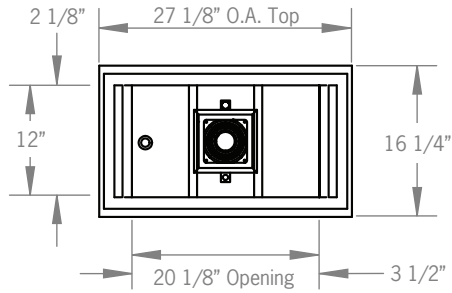
KRD-27S Plan View
