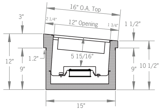
Raised Rail Section View
