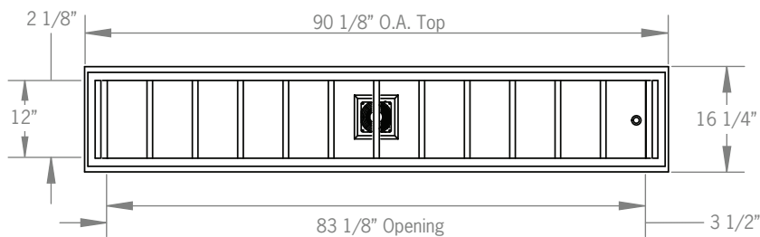
KRD-90S Plan View
