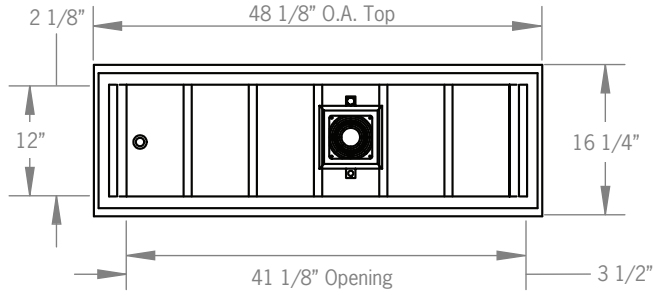
KRD-48S Plan View
