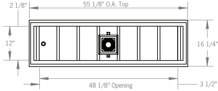
KRD-55S Plan View
