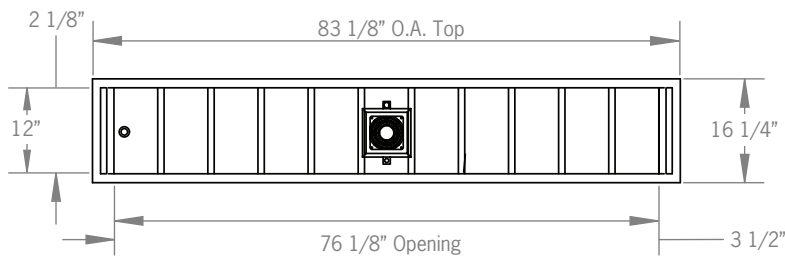
KRD-83S Plan View
