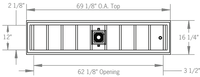
KRD-69S Plan View
