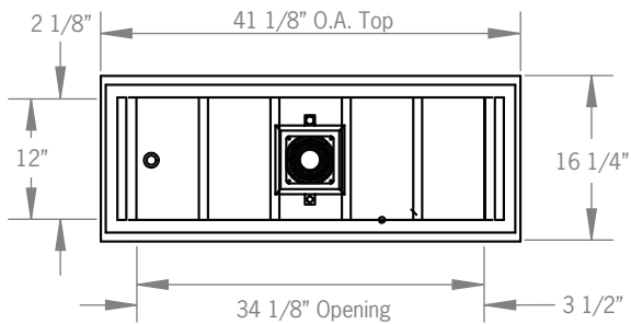
KRD-41S Plan View
