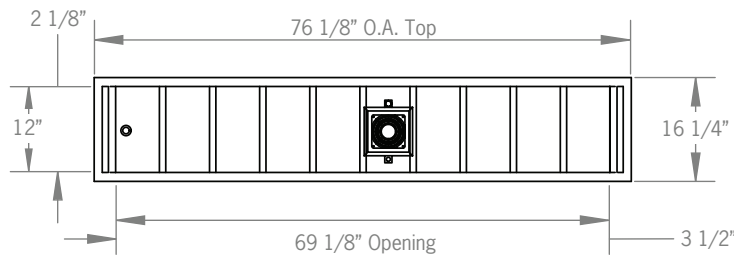
KRD-83S Plan View
