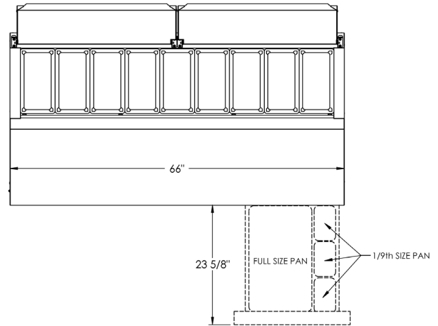
Plan & Elevation View - KS066
