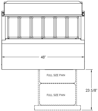
Plan & Elevation View- KS048
