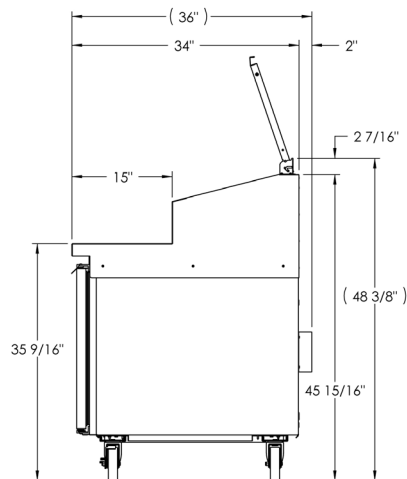
Section View - All Models
