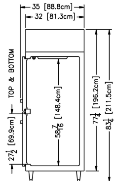
Section - R/ALT232DUT
