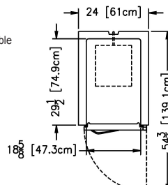
Plan - R/ALT132DUT
