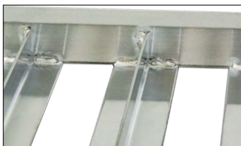
Closeup: Underside of T-Bar Shelf.
